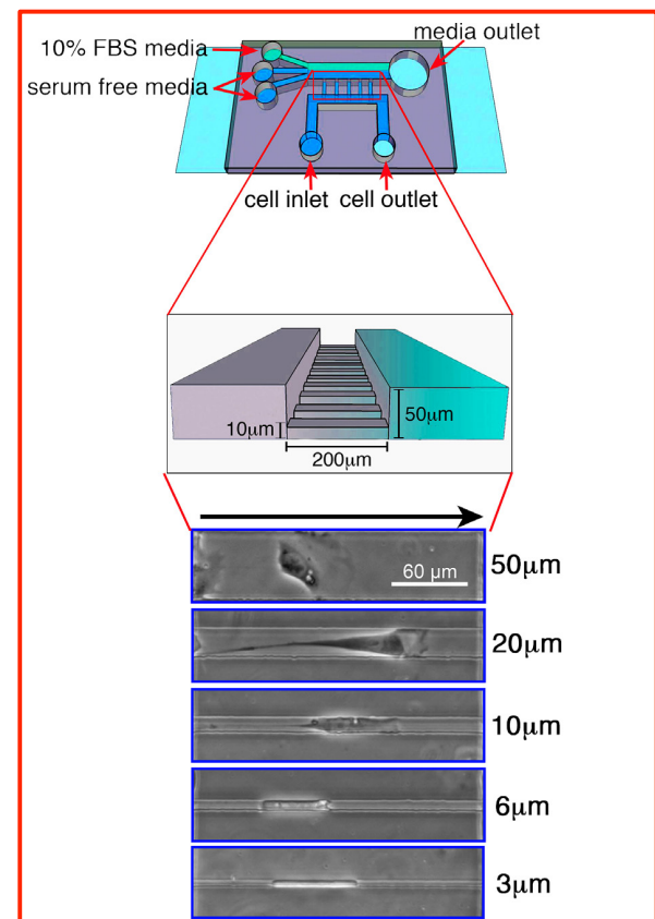
Illustration of the micro-channel array device.
